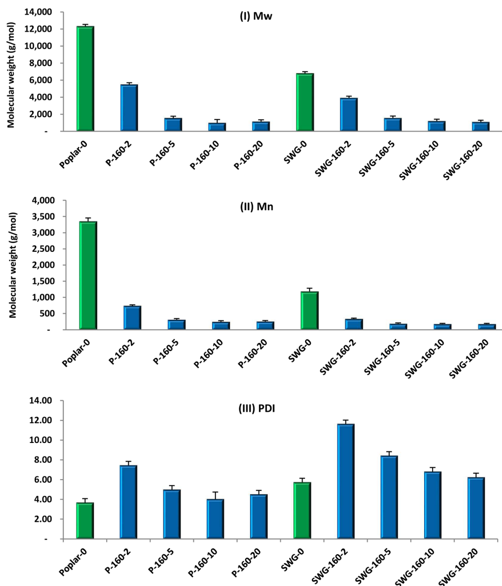
Figure 1. Molecular weight change of cellulosytic enzyme lignin (determined as acetate) after DAP at various residence time. (I) Weight-average molar mass ( M_w ), (II) number-average molar mass ( M_n ), and (III) polydispersity index (PDI).
